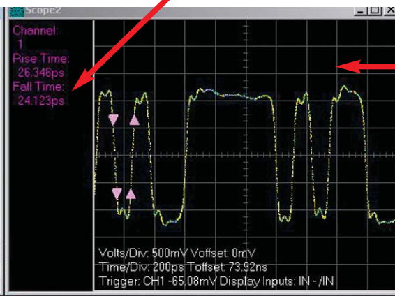
Fast Rise/Fall Times
